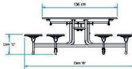
End View
